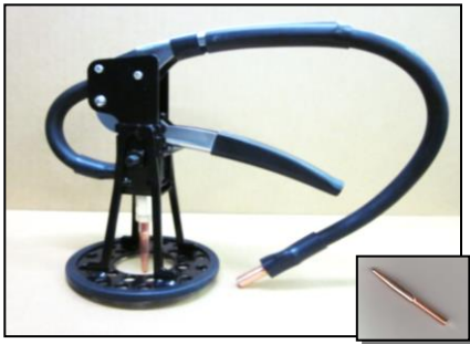
Handy Puller
